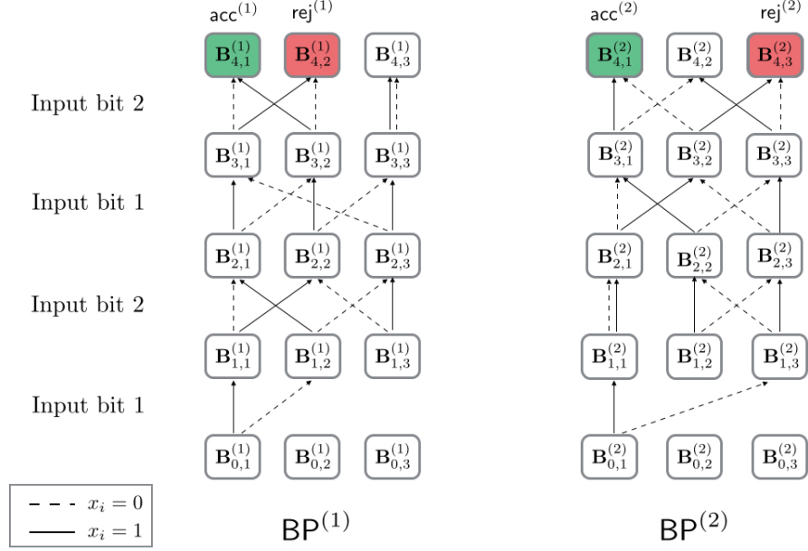
Fig. 1: Branching programs \text{BP}^{(1)} and \text{BP}^{(2)} .
