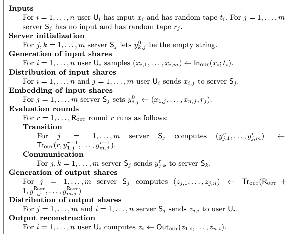
Fig. 3. Running an outer protocol \pi_{\text{OUT}} = (R_{\text{OUT}}, \text{In}_{\text{OUT}}, \text{Tr}_{\text{OUT}}, \text{Out}_{\text{OUT}}) for f
