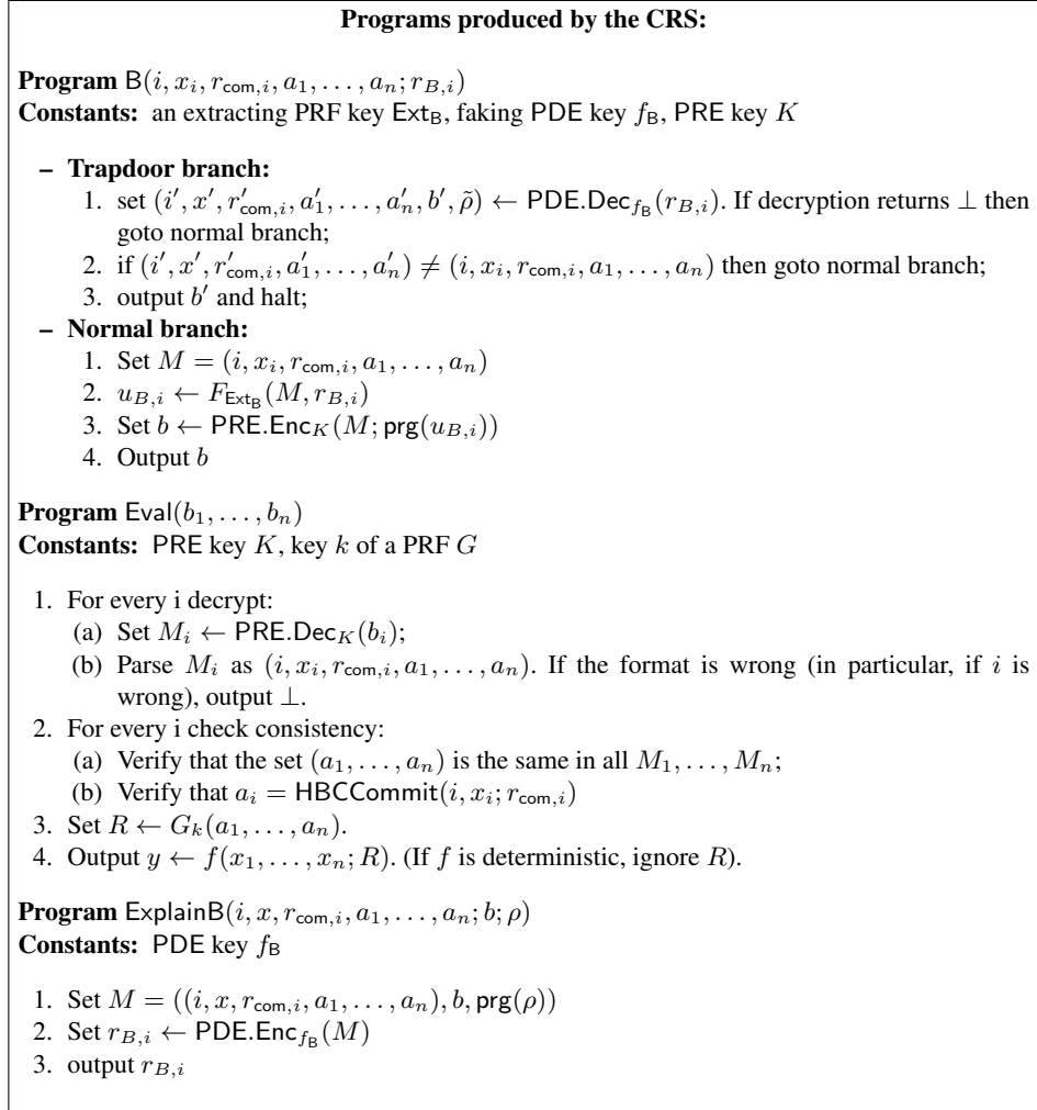
Fig. 4: Programs used in the protocol.
