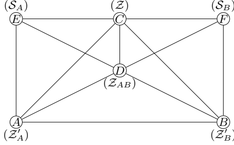
Fig. 4. H_{OT}(\mathcal{V}_{H_{OT}}, \mathcal{E}_{H_{OT}}) : OT between A and B with security w.r.t. malicious adversary structure \{\{C\}, \{A, D\}, \{B, D\}\} is impossible (Lemma 5). The sets shown inside brackets correspond to the vertex identification used in the proof of Lemma 6.
