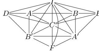
Fig. 10. In the full version [33], we show the necessity of the second condition for the general case by showing the impossibility of OT between A and B in this graph with statistical security w.r.t. the malicious adversary structure \{\{C\}, \{A, A', I\}, \{B, B', I\}\} .
