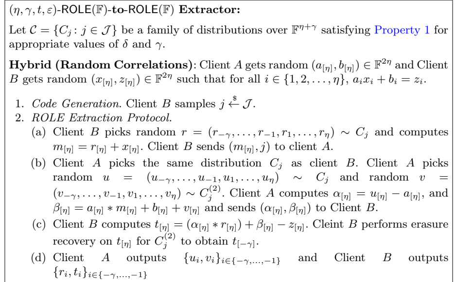
Fig. 4. \text{ROLE}(\mathbb{F}) -to- \text{ROLE}(\mathbb{F}) Extractor Protocol.
