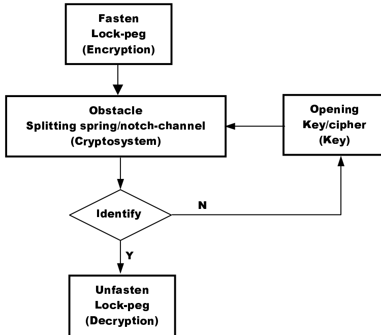
Fig. 3. Cryptosystem of Chinese locks
