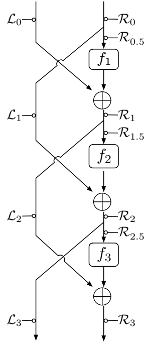
Fig. 1. An illustration of A_3 ; the locations at which to XOR a tweak of length |M|/2 for 3-round LR.
