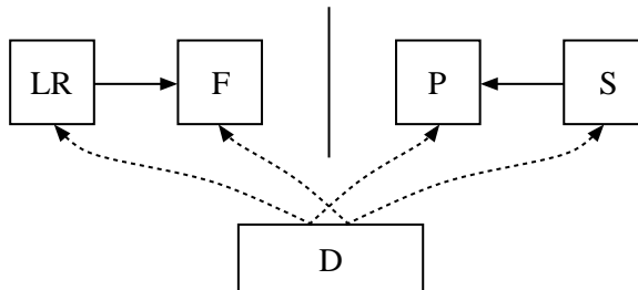
Fig. 3. The indiffereniability notion.
