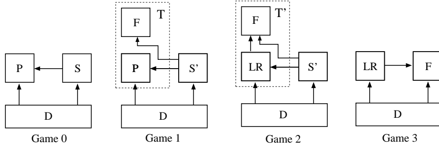
Fig. 5. Sequence of games for proving indifferentiability.
