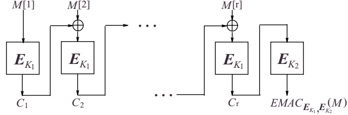
Fig. 3. The EMAC algorithm
