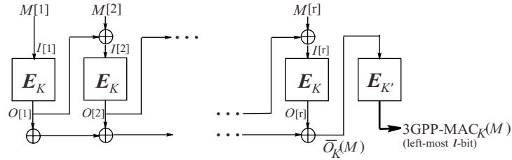
Fig. 1. The 3GPP-MAC algorithm
