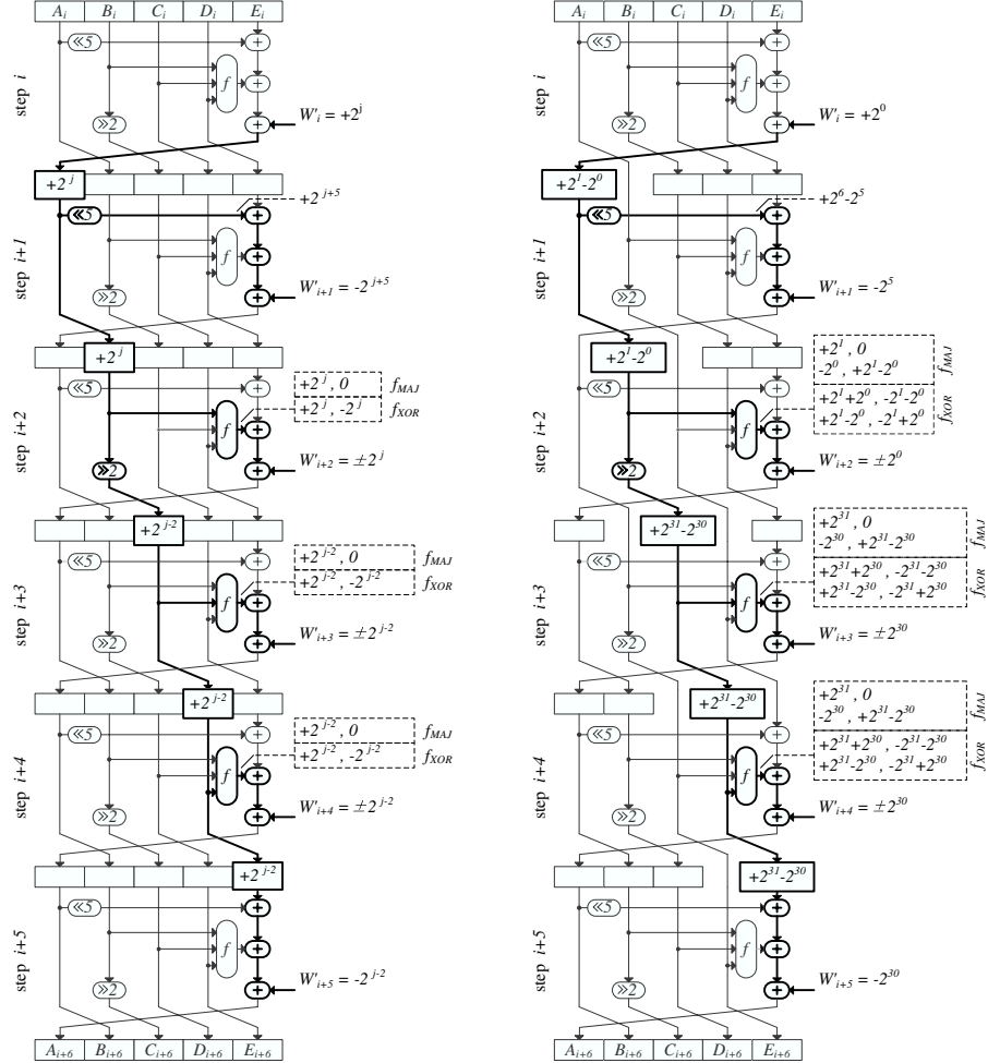
Fig. 3. On the left, a local collision with disturbance in bit position j . No carry occurs in step i . On the right a local collision with disturbance in bit position j = 0 . In step i a carry occurs. The differences in the dashed rectangles are the possible output differences of f_{XOR} and f_{MAJ}
