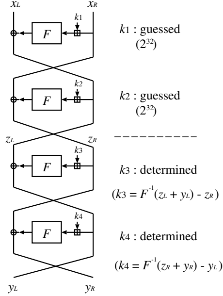
Fig. 6. Equivalent keys of 4 rounds
