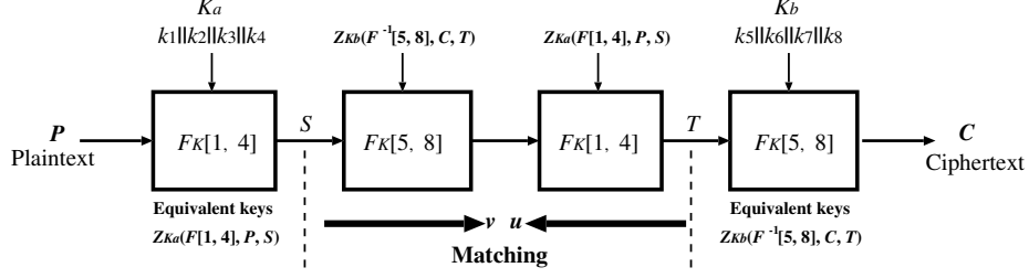
Fig. 7. R-MITM stage using equivalent keys
