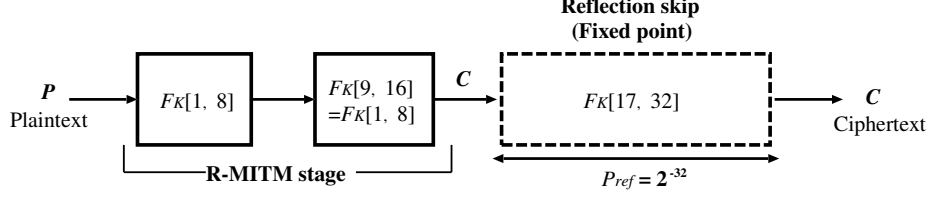
Fig. 5. Reflection skip of GOST
