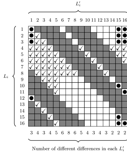
Figure 5: A ✓ means we know both value and difference for that byte, a ● means that we only determined the difference for that byte and white bytes are not constrained yet.
