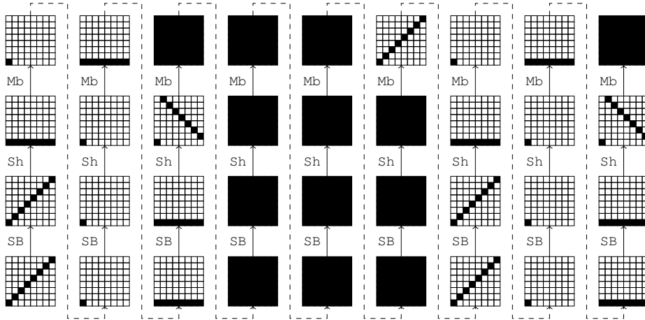
Figure 7: The 9-round truncated differential characteristic used to distinguish the permutation P of Grøstl-256 from an ideal permutation.
