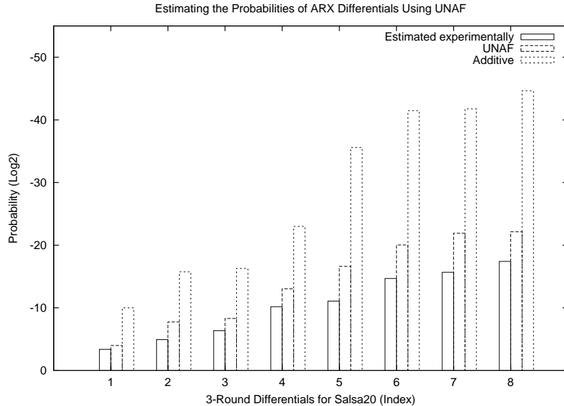
Fig. 4. Three estimates of the probabilities of eight differentials for three rounds of Salsa20, based on the data from Table 4: (1) estimation obtained experimentally, (2) based on UNAF differences and (3) based on single additive differences.
