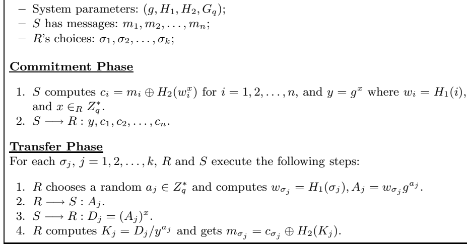
Fig. 3. Adpt-OT _n^k : Adaptive OT _n^k
