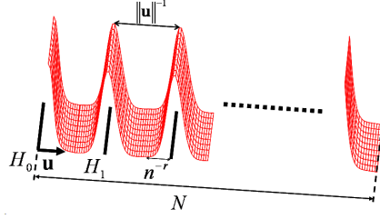
Fig. 2. ciphertexts of 0 in \text{AD}_{\text{GGH}}
