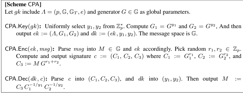
Fig. 5. The Linear Encryption Scheme.
