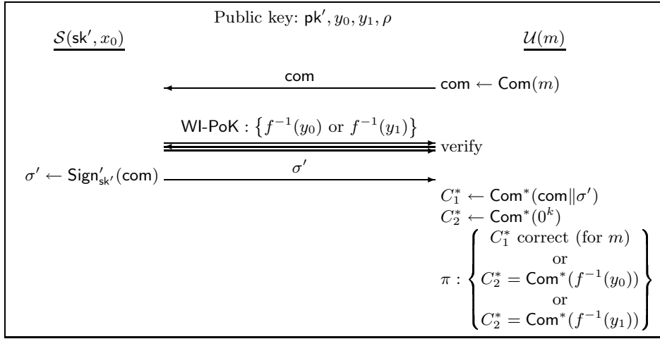
Fig. 2. A partial solution using complexity leveraging.
