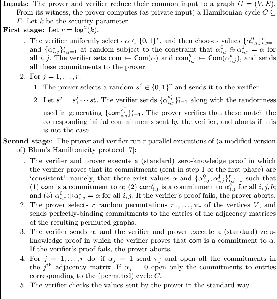
Fig. 3. A concurrent zero-knowledge argument of knowledge.
