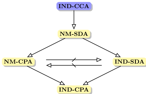
Fig. 1. Diagram of the main relationships between the security notions considered in this paper. X \rightarrow Y means that X implies Y ; X \nrightarrow Y indicates a separation between X and Y . Notions with the same color are equivalent under black-box transformations; notions with different colors are not known to be equivalent.
