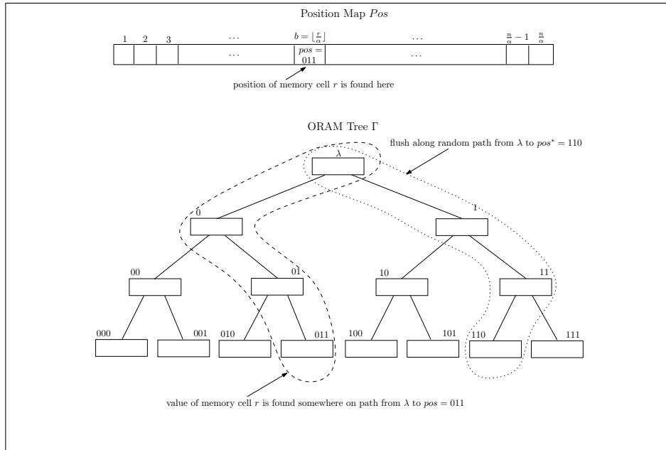
Fig. 1: Illustration of the basic [CP13] ORAM construction.
